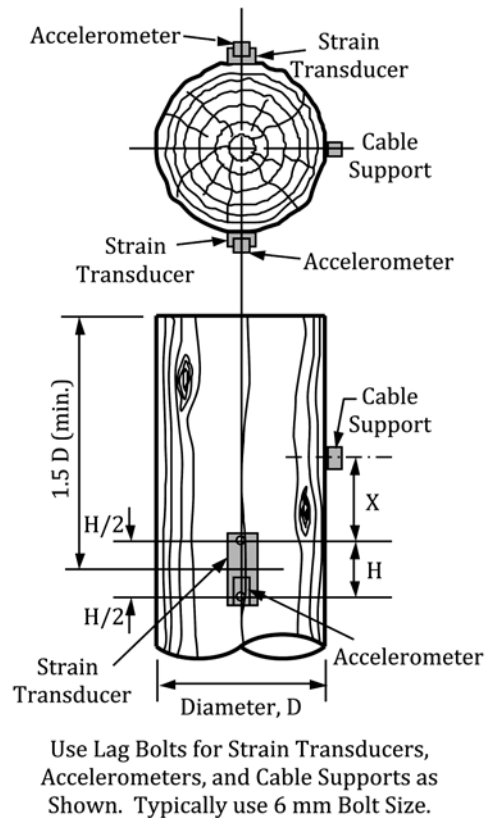
FIG. 6 Typical Arrangement for Attaching Transducers to Wood Piles
